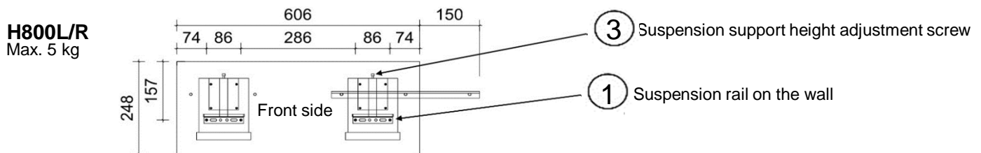
Drilling dimensions of wall shelf outer edges for suspension rails
