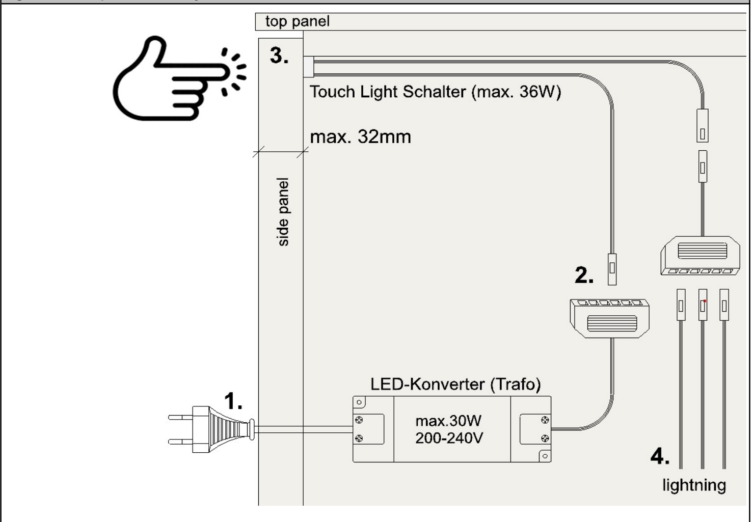
Figure 1: Example of assembly behind the furniture
