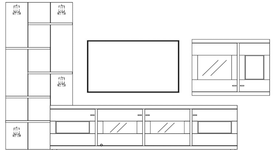
Panel - hanging lowboard cut-out, NE16 L
